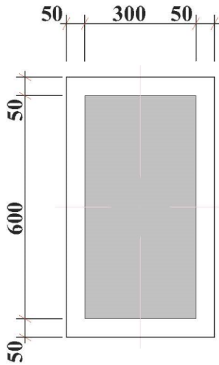
COLUMN COPING SCALE 1:10
