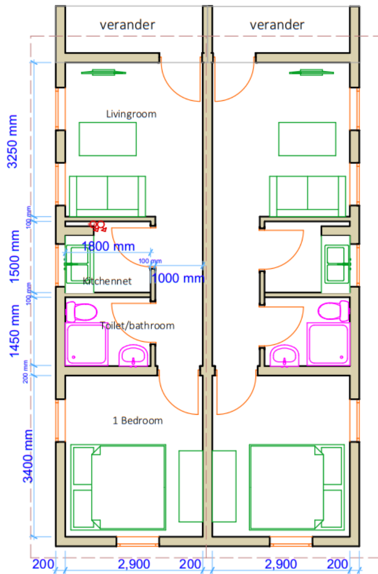
One Bedroom Type A
